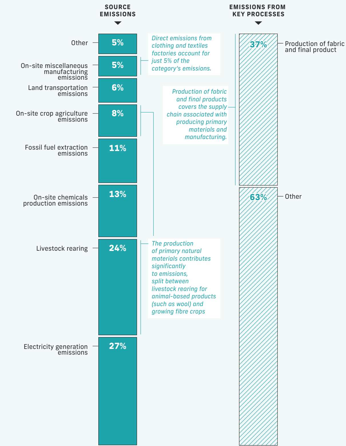
fig.20 Source emissions of clothing and textiles during the period 2017-2050 under an NDC scenario.
