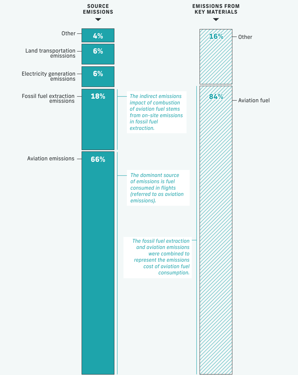
fig.24 Source emissions from flights from 2017-2050 under an NDC scenario.
