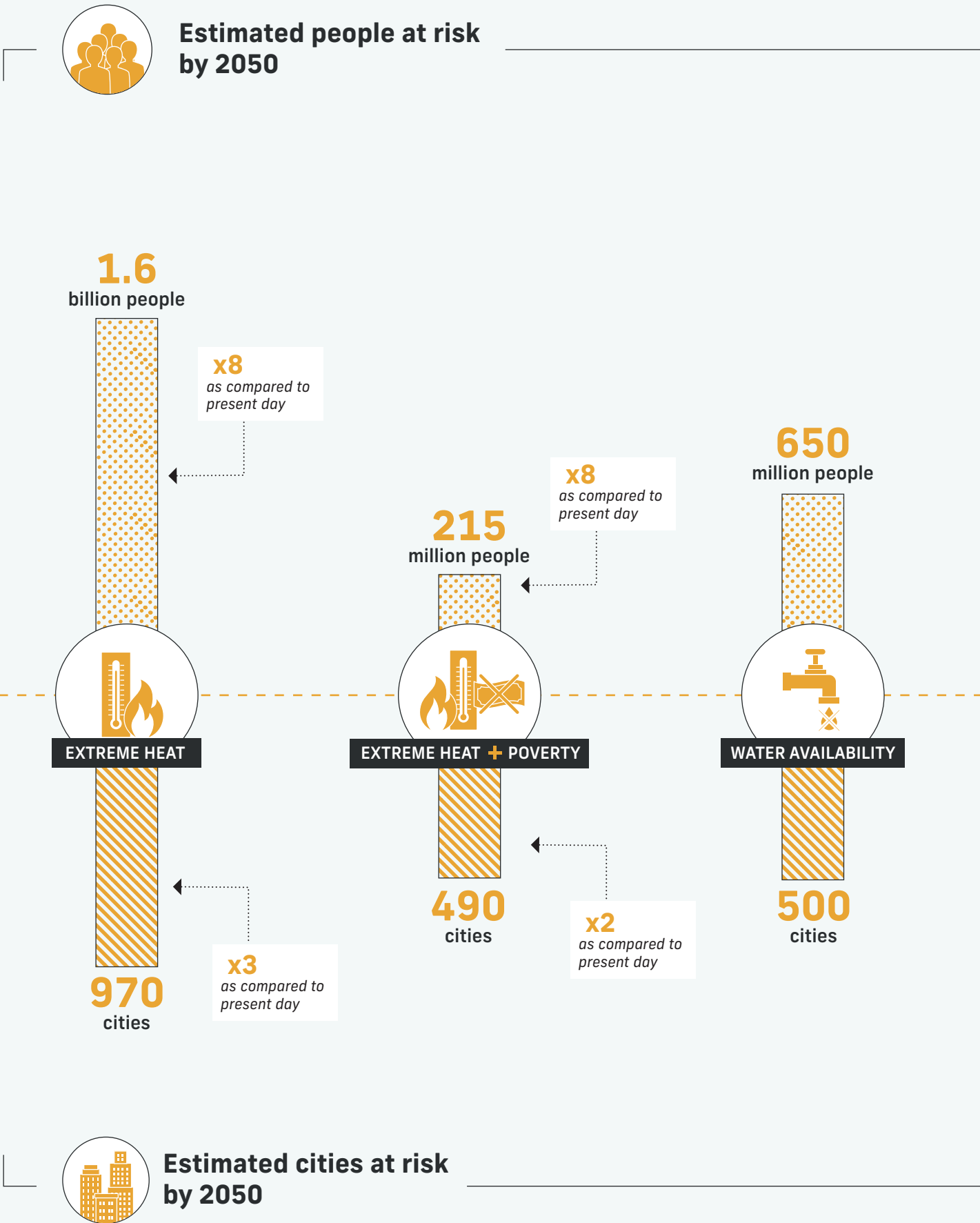
fig.1 A summary of critical risks A summary of critical risks that cities and their residents will encounter as a result of climate change.
